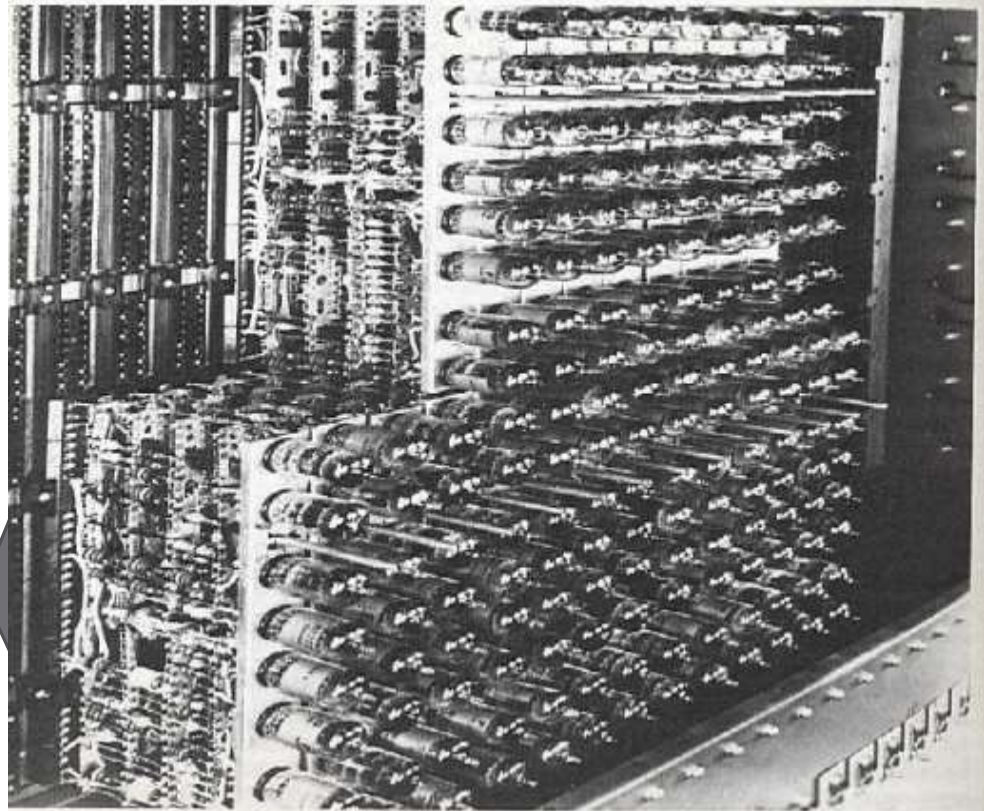
IBM 701 panel
