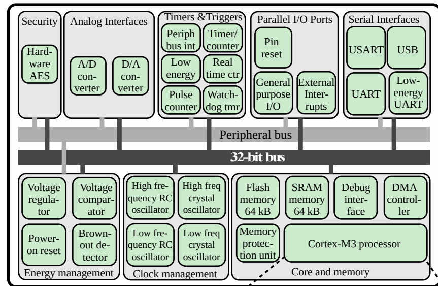
Microcontroller Chip
